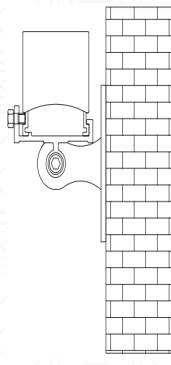
Wall installation
