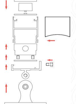
Product Teardown Diagram
